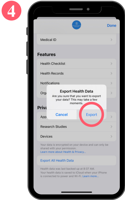
4) Confirm export
