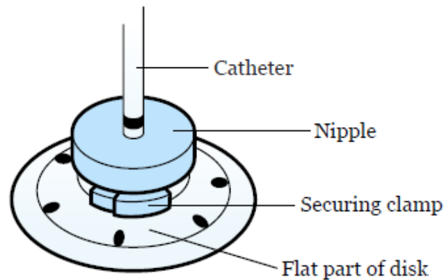
Figure 7. Silicone disk over catheter
