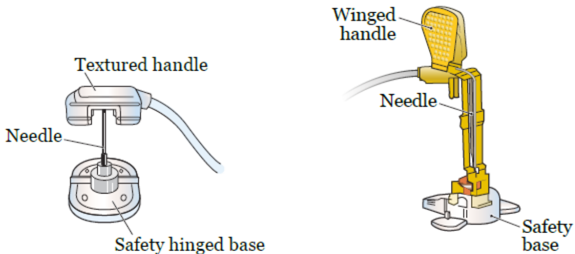
Figure 2. Examples of needle in locked safety position
