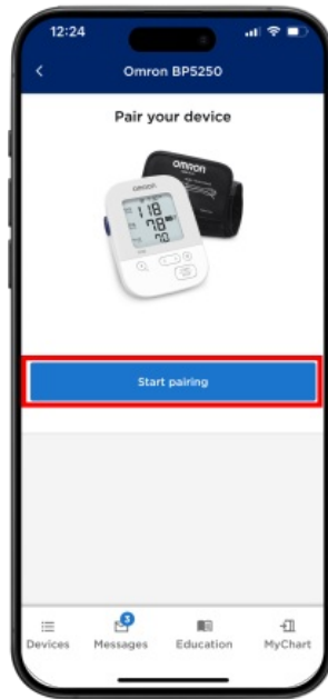
Figure 6. Start pairing
