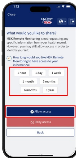
Figure 3. Allow access
