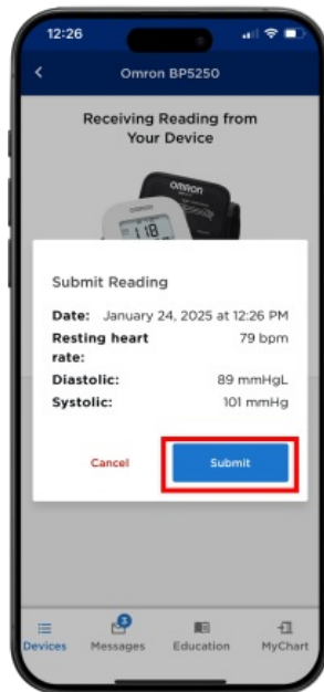
Figure 11. Submit reading
