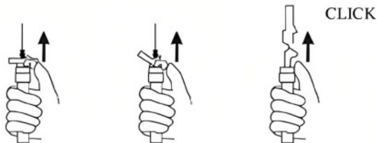
Figure 7. Pushing the LuproLoc safety device into place
