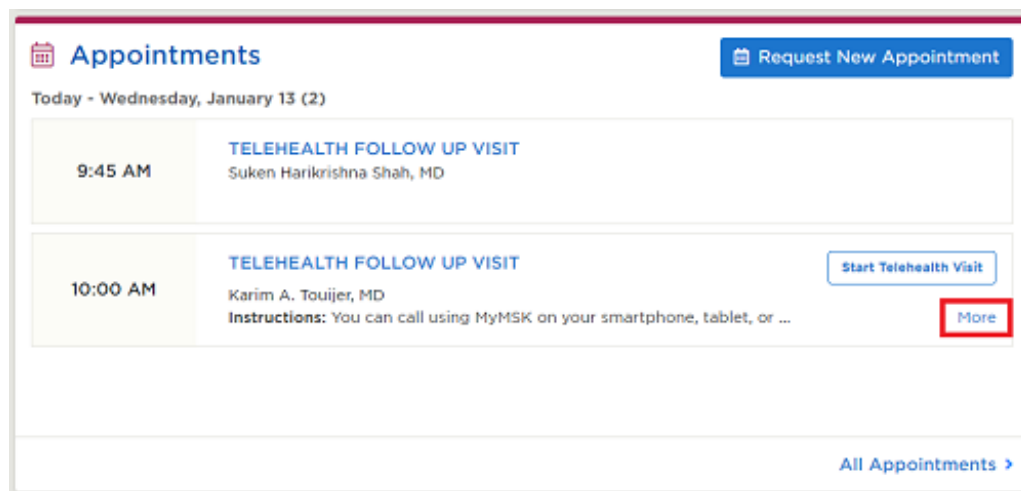
Figure 2. Select “More”
